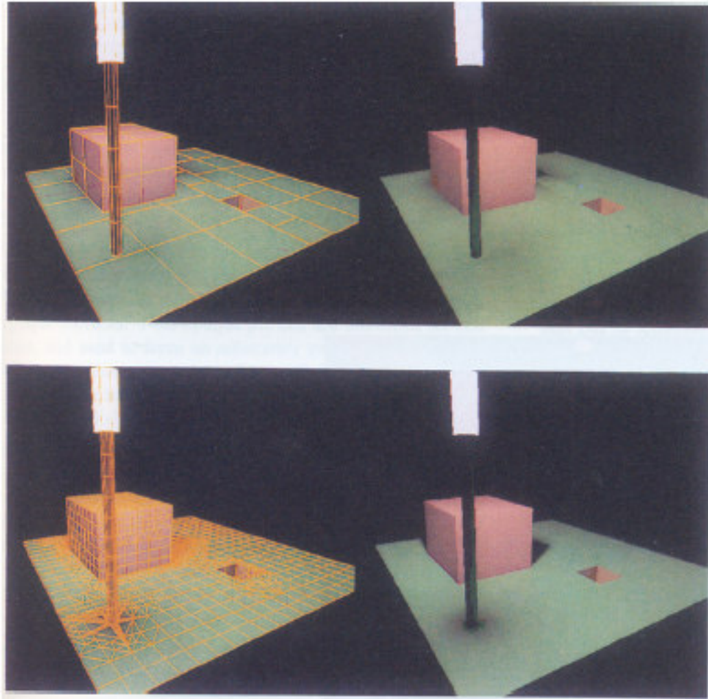
Fig11. Radiosity rendering for octree model.
